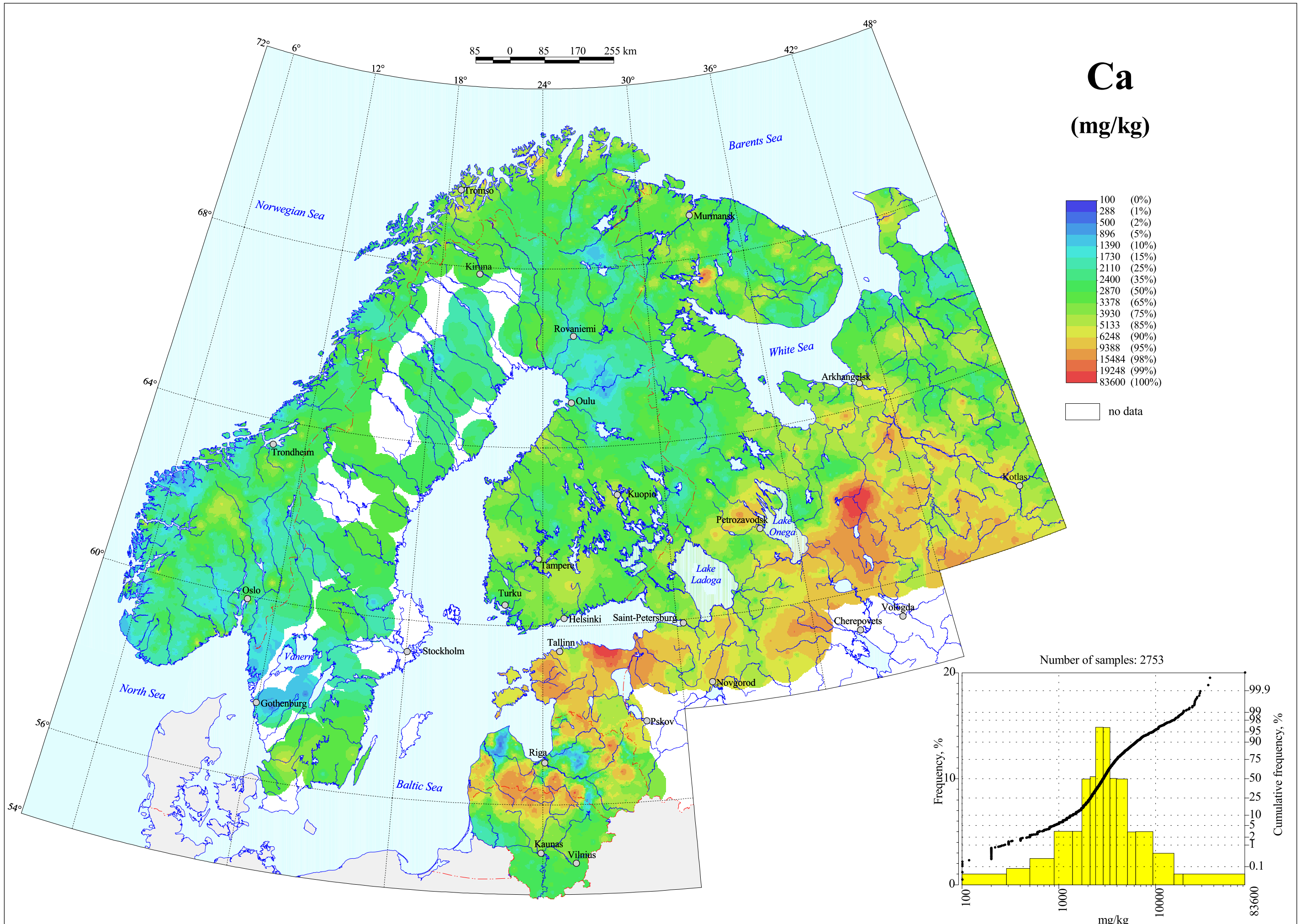
Calcium in Organic Soil Layer, Total Content
